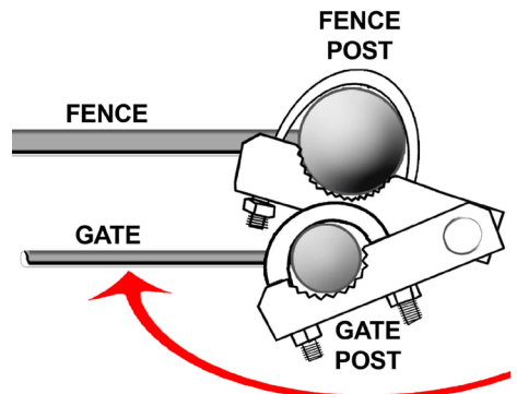
Chain Link - 180° Gate Hinge
